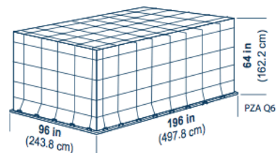
IATA ULD code: PZA Q6 Universal general-purpose flat pallet for lower holds and main decks.
