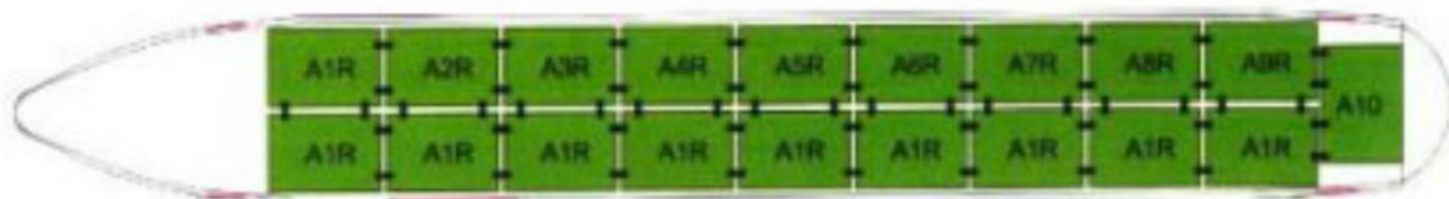
CONFIGURATION A 125" X 88" SIDE BY SIDE - ULD LAYOUT
