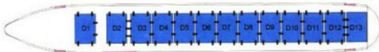
CONFIGURATION D 88" X 125" CENTERLINE - ULD LAYOUT
