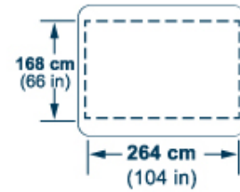
Forward lower cargo compartment door (STA 615)
