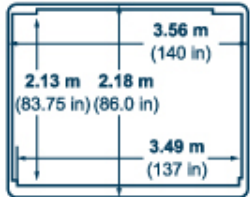
Main deck cargo door
